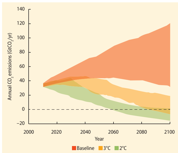
FIGURE 6.5 Carbon neutrality is needed by 2100 to achieve climate goals
