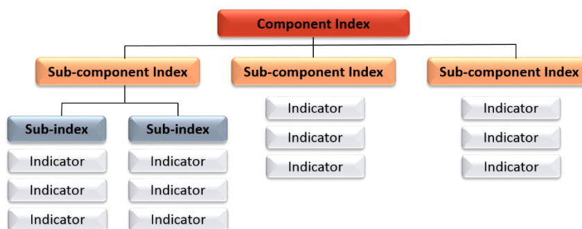
Figure 6. Index hierarchy
