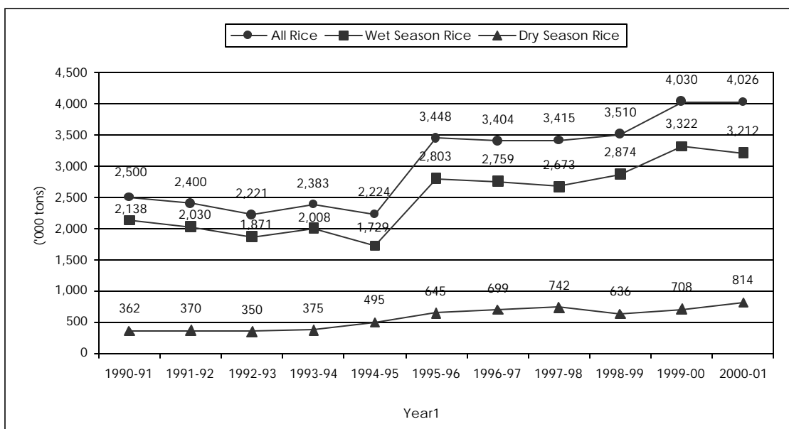
Figure 2.1: Rice Production, 1990-2001
