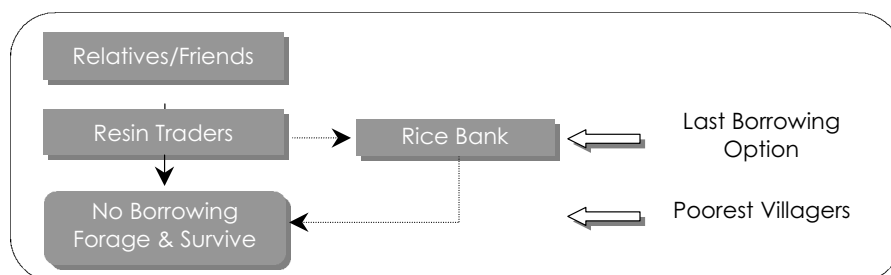
Figure 3.4: Hierarchy of Borrowing Strategies
