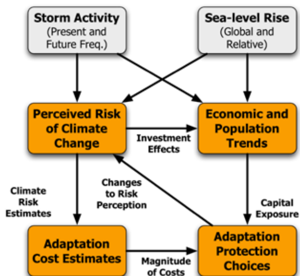
Figure 8.1: The Feedback-Rich Adaptation to Climate Change (FRACC) Model
