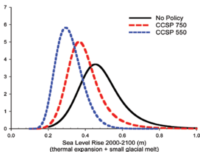
Figure 8.8: Probability density function showing joint program SLR estimates
