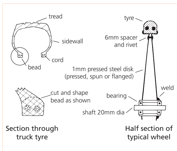
Figure 6.5 A simple handcart tyre made from the bead of a used truck tyre
