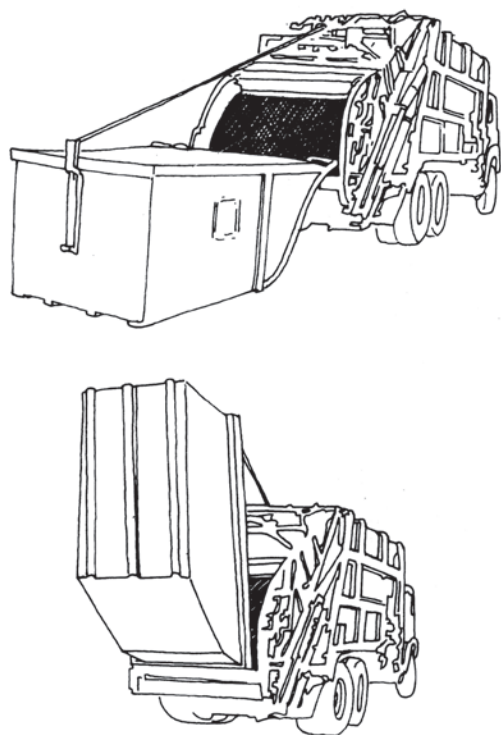
Figure 7.23 Large rear-loading compactor truck emptying large skip container
