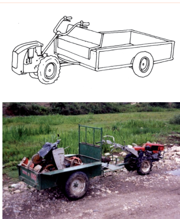
Figure 7.6 and Photo 7.6 Low-cost two-wheel tractor adapted for waste collection
