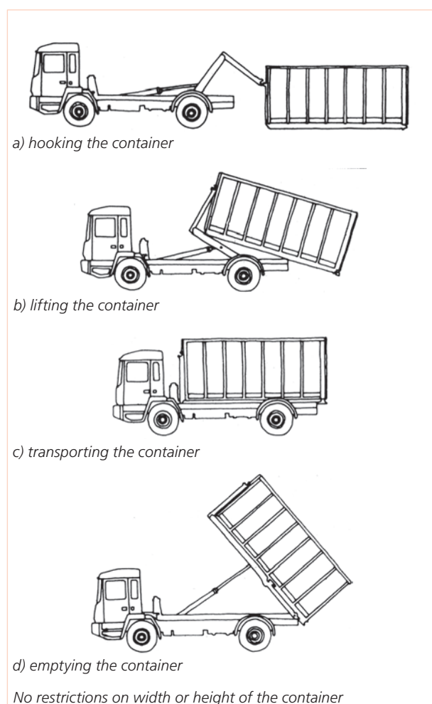
Figure 7.34 Hooklift system
