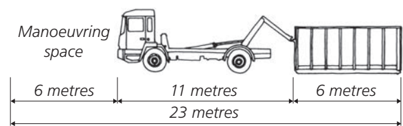
Figure 7.35 A hooklift truck to carry a 6 m long container requires a minimum clear space of 23 metres by 6 metres to allow for depositing an empty container and picking up a full one.
