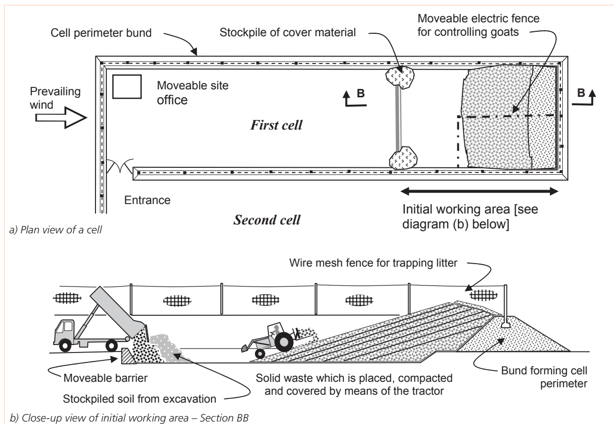
Figure A5.4 Proposal for constructing and operating a cell in a small landfill
