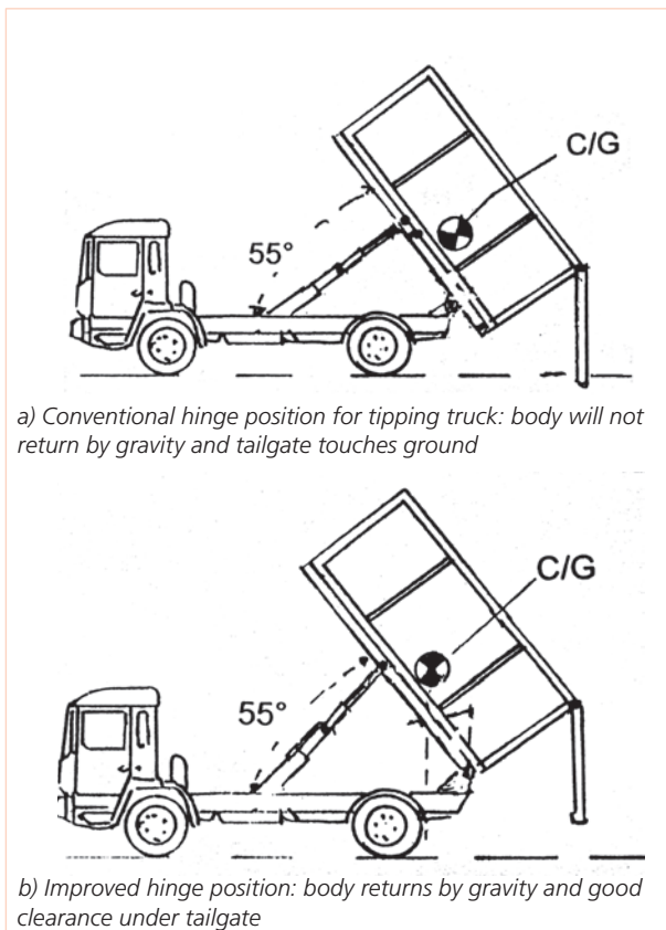
Figure 7.10 The location of the point at which the body is hinged to the chassis is an example of a design detail that can have a major impact on the operation of a vehicle
