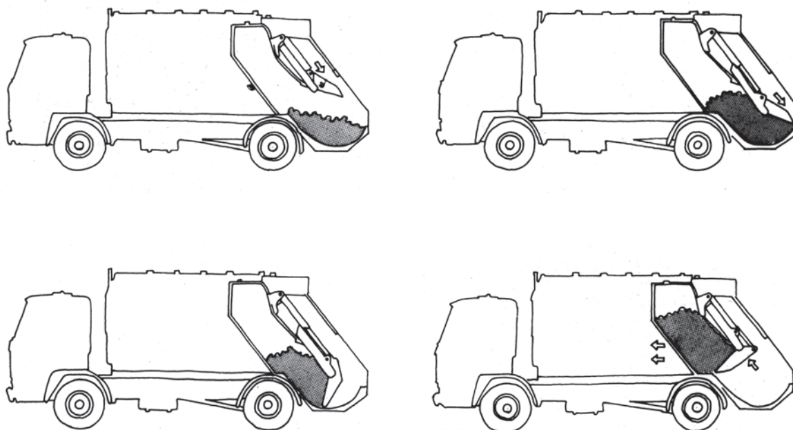
Figure 7.22 Rear-loading compaction plate compactor. Suitable for low-density waste including large items and for use with binlift. Intermittent loading.
