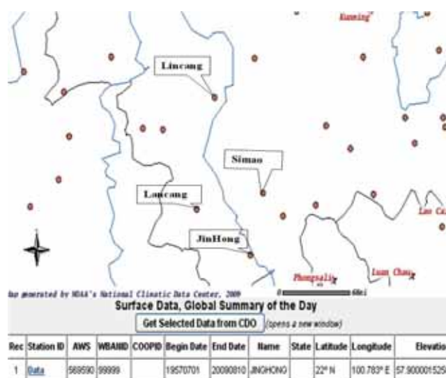
Fig. 1 Selected rainfall stations in the Upper Mekong Basin in Southern Yunnan. ( http://www7.ncdc.noaa.gov/CDO/cdosubqueryrouter.cmd )
