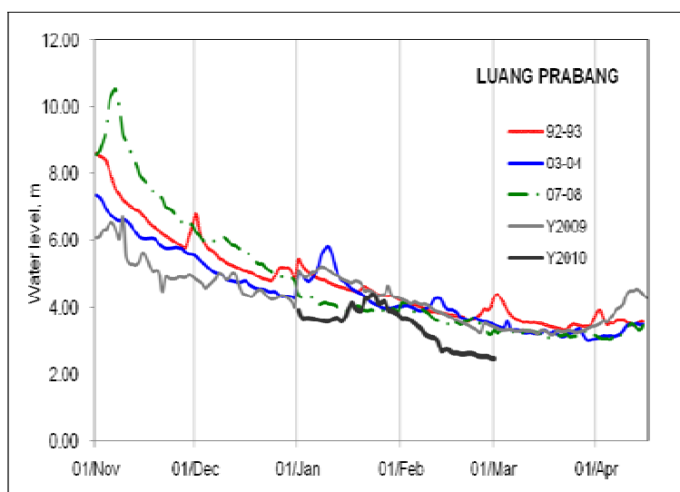
Fig. 6 Chiang Saen, Luang Prabang, Vientiane and Kratie: Water levels of 01 November 2009 – 28 February 2010 compared to those 1992-93, 2003-04 and 2007-08
